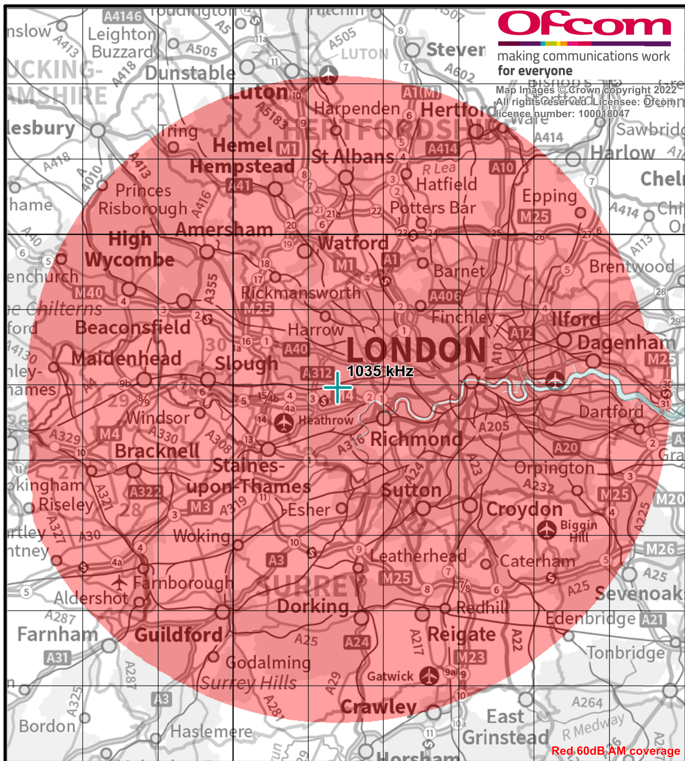
London AM4 (Lyca Dil Se 1035) coverage area - 23rd June 2021
