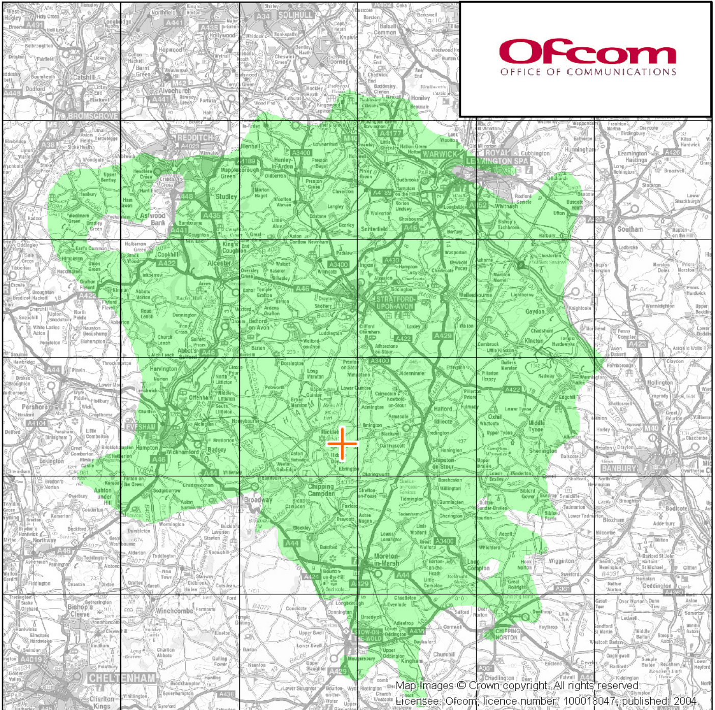
Stratford FM MCA (FM 102 - The Bear) - 29th December 2003
