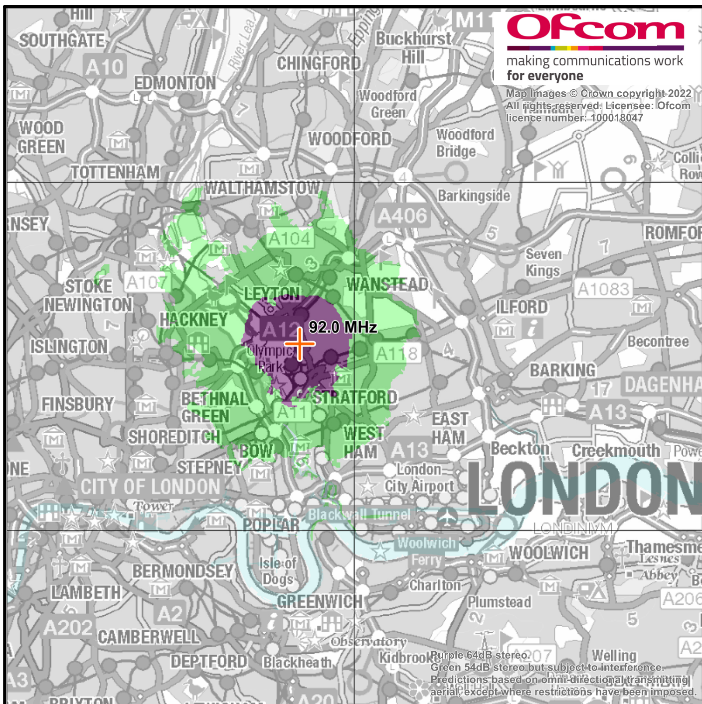
London - Forest Gate (Nu Sound Radio) community radio coverage area 1st September 2021
