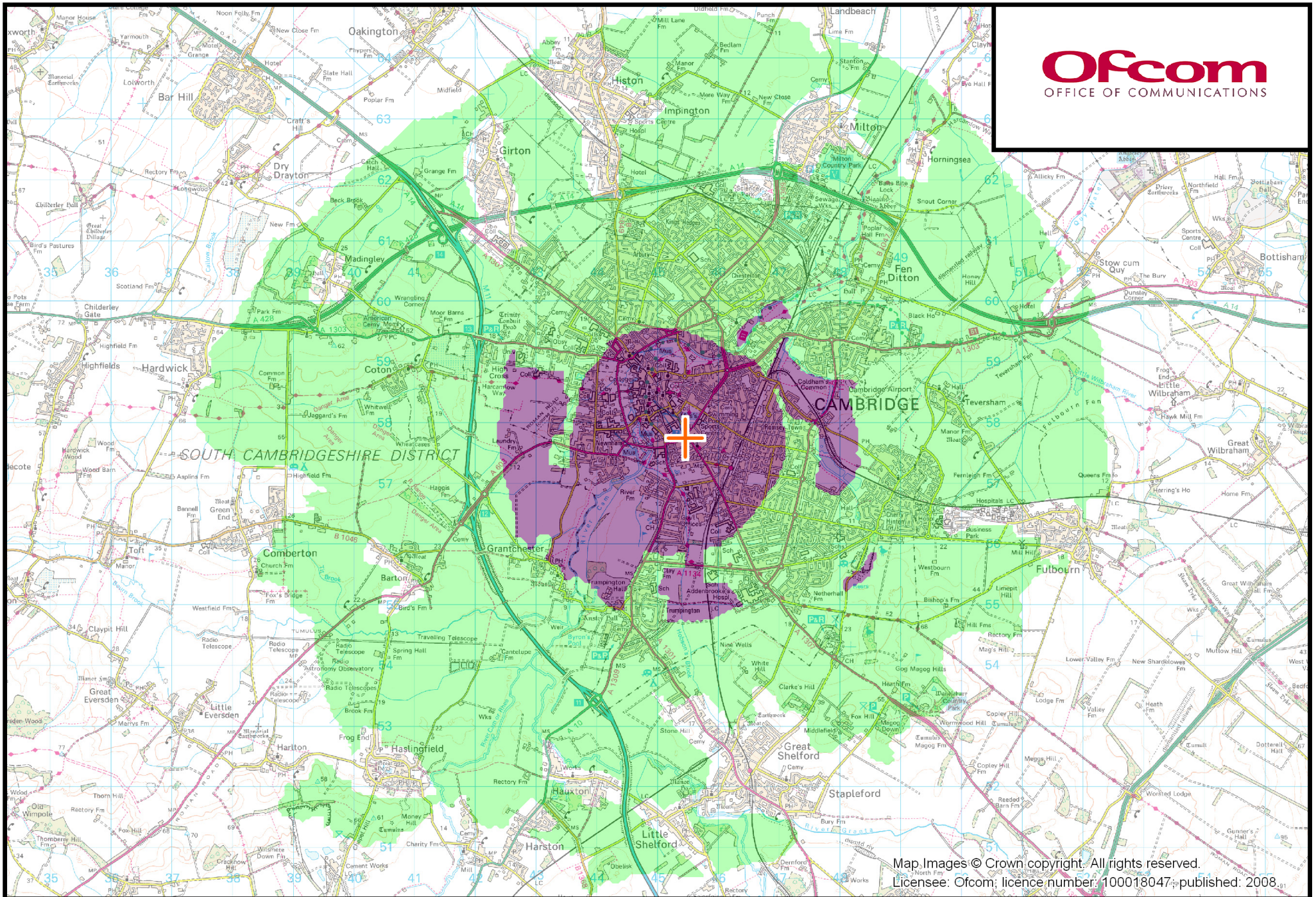
Cambridge community radio coverage area - 28th September 2007
