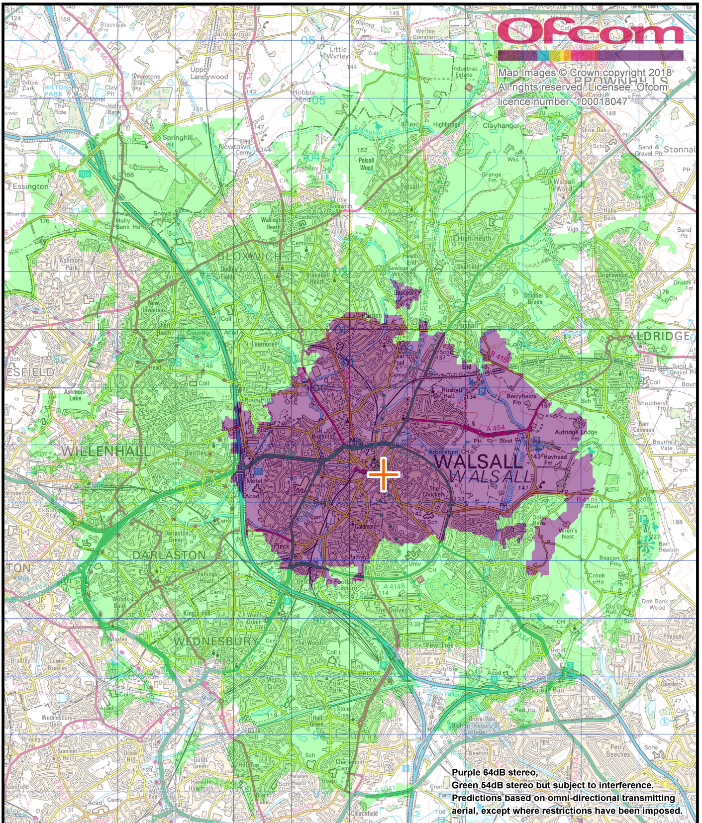
Walsall (Ambur Radio) community radio coverage area - 9th March 2016
