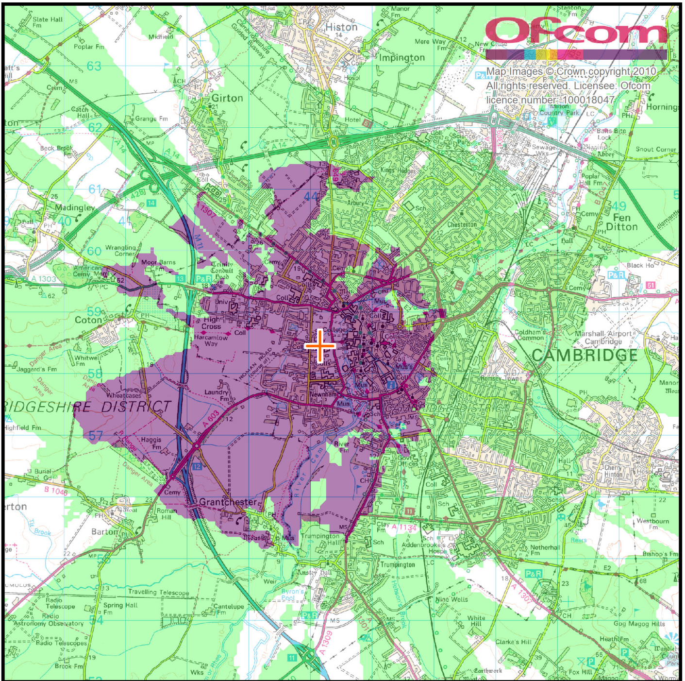
Cambridge (CAM FM) community radio coverage area - 28th September 2010
