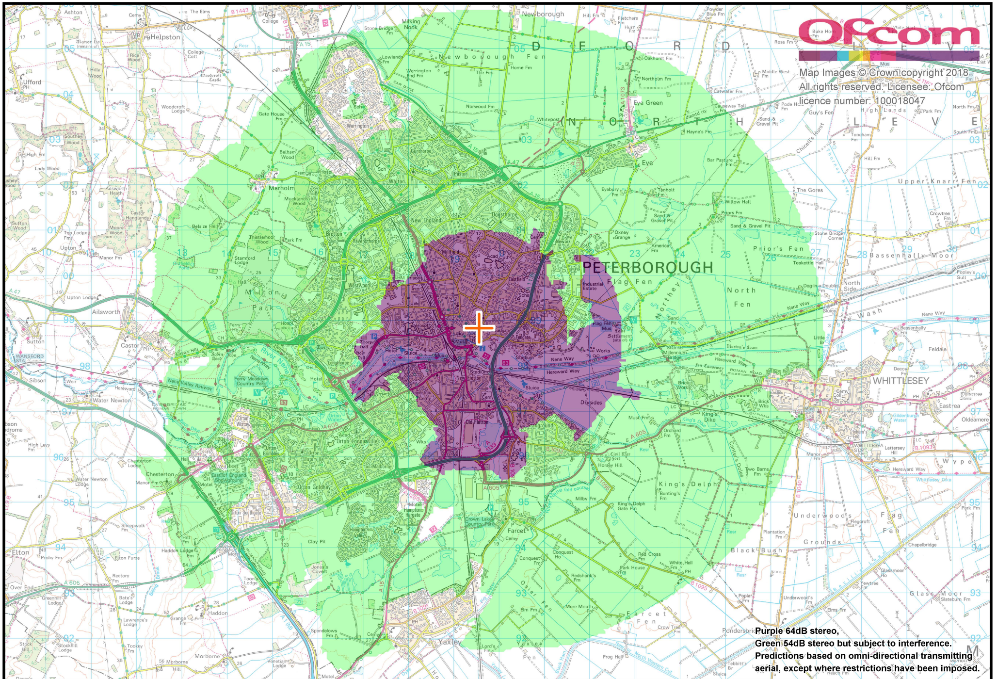
Peterborough (Salaam Radio) community radio coverage area - 7th June 2016
