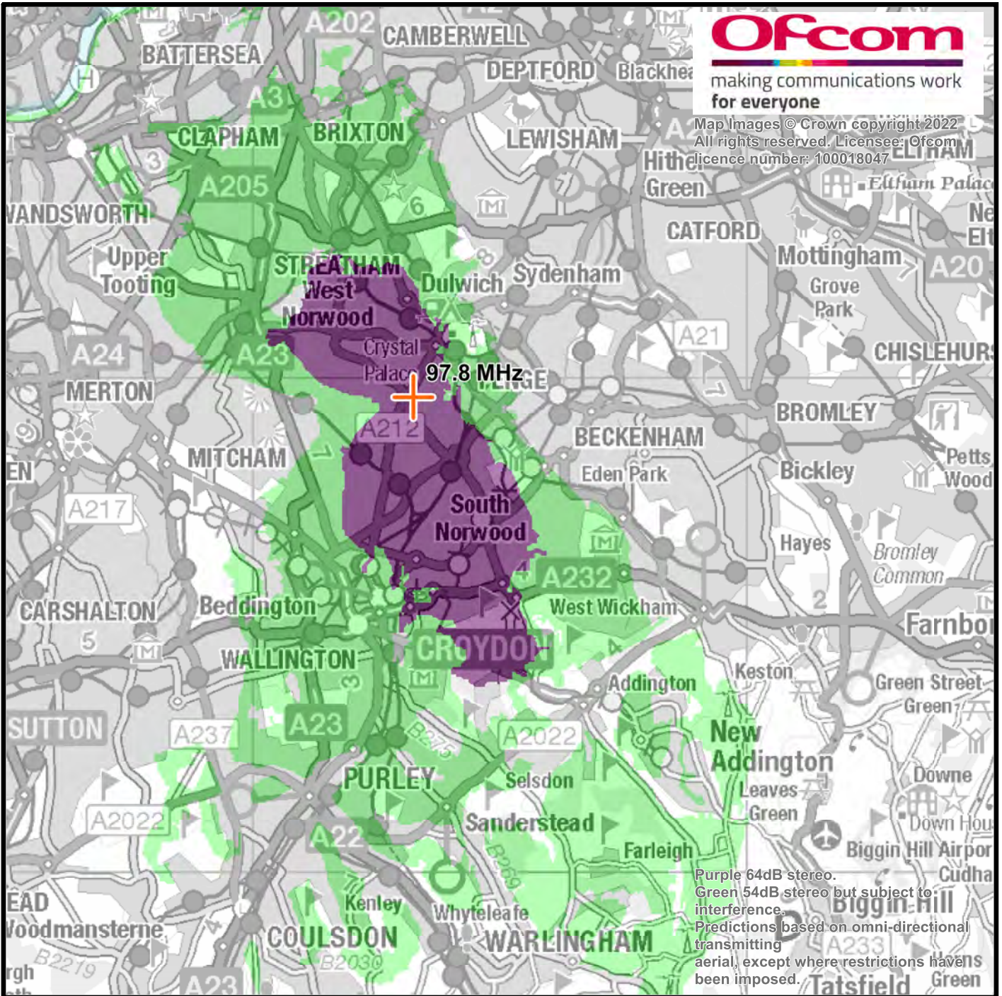
Croydon (Croydon FM) community radio coverage area - 9th September 2021
