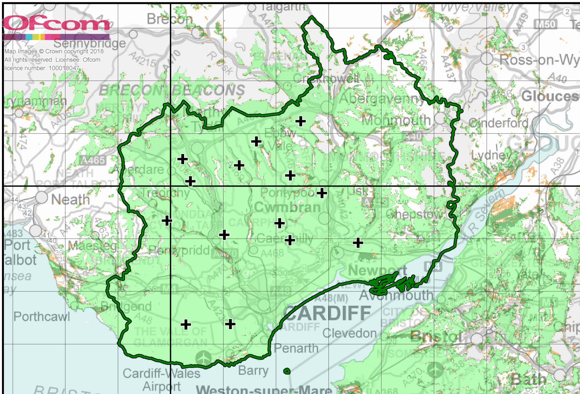
South East Wales local DAB multiplex service (NowDigital). Indoor coverage, enhanced propagation conditions. July 2018.
