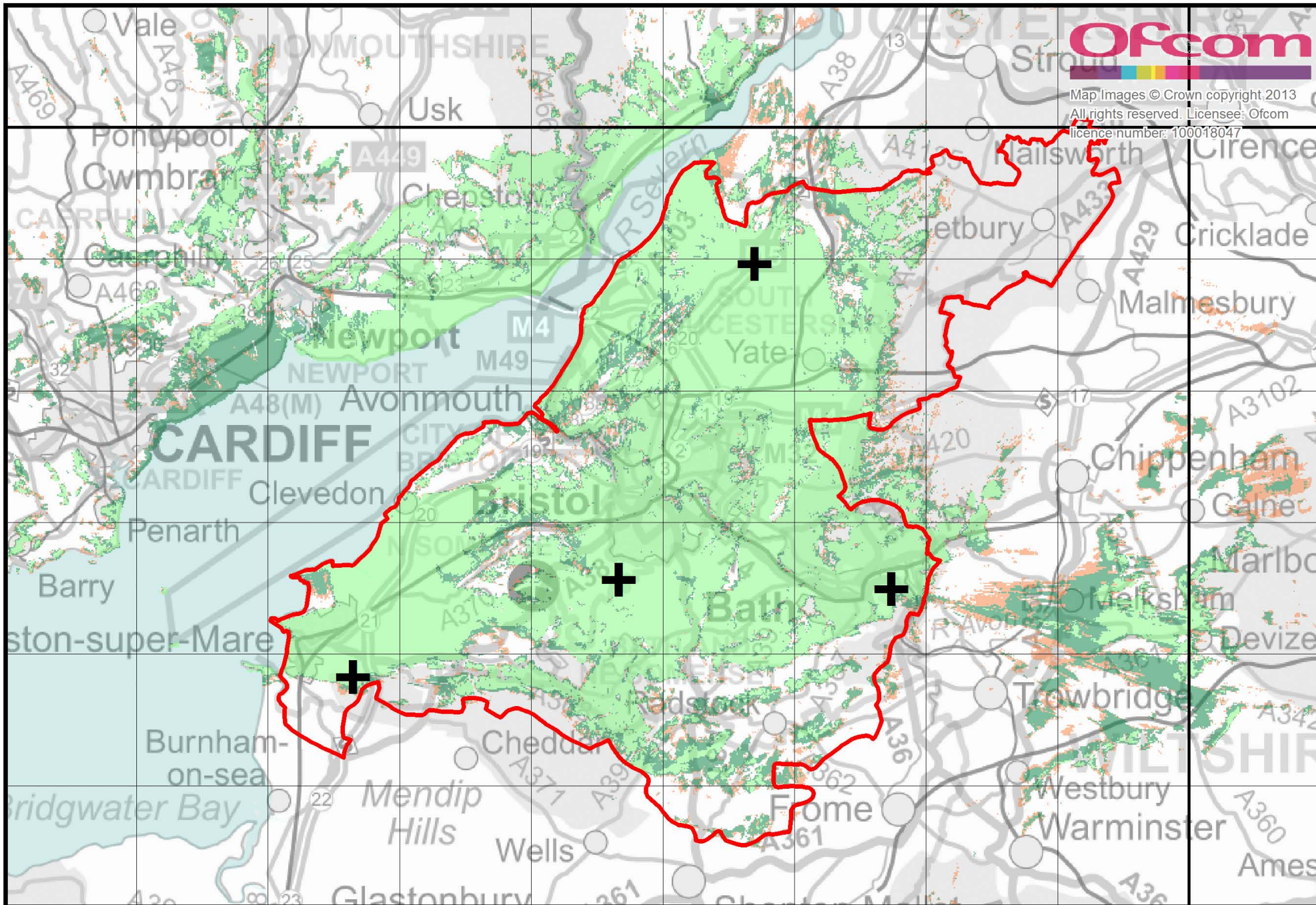
Bristol and Bath local DAB multiplex service (NOW Digital) indoor coverage enhanced propagation conditions, January 2013
