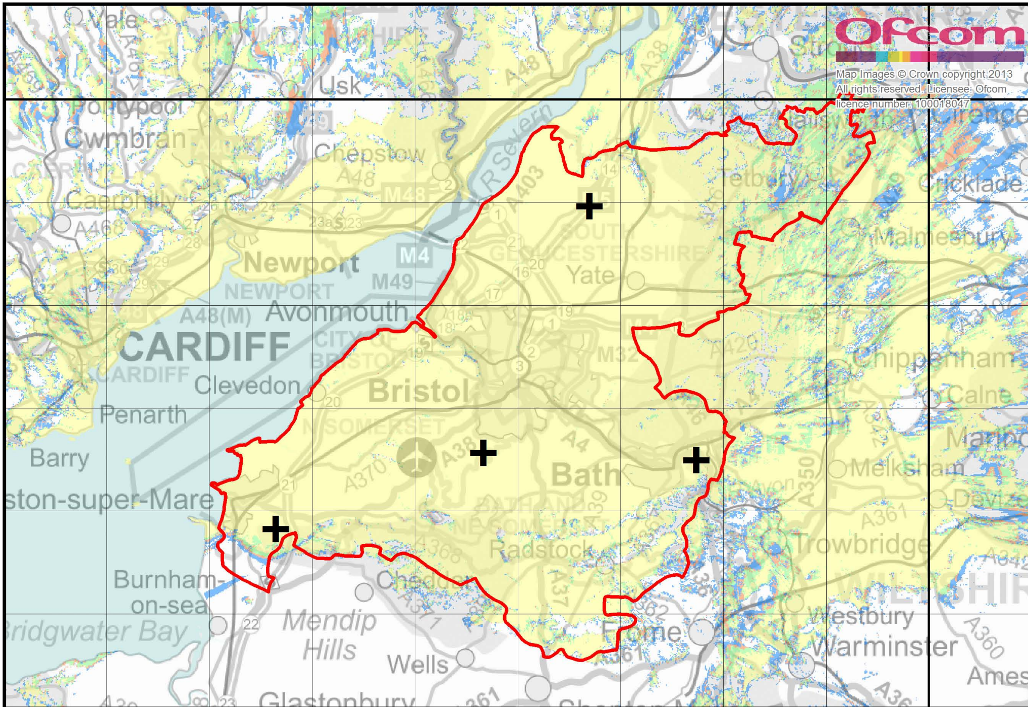
Bristol and Bath local DAB multiplex service (NOW Digital) mobile coverage normal propagation conditions, January 2013
