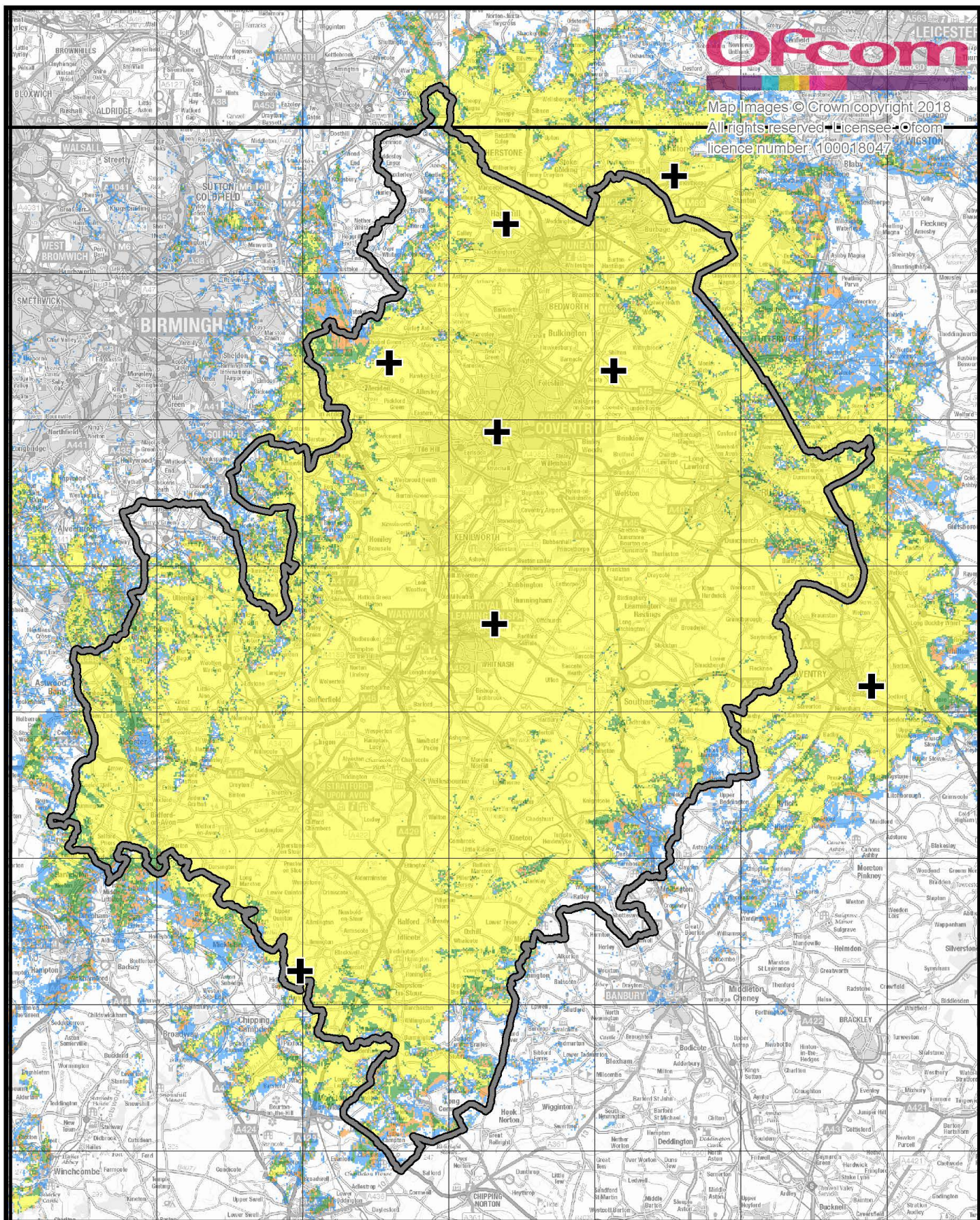
Coventry local DAB multiplex service (Now Digital). Mobile coverage, enhanced propagation conditions. July 2018.
