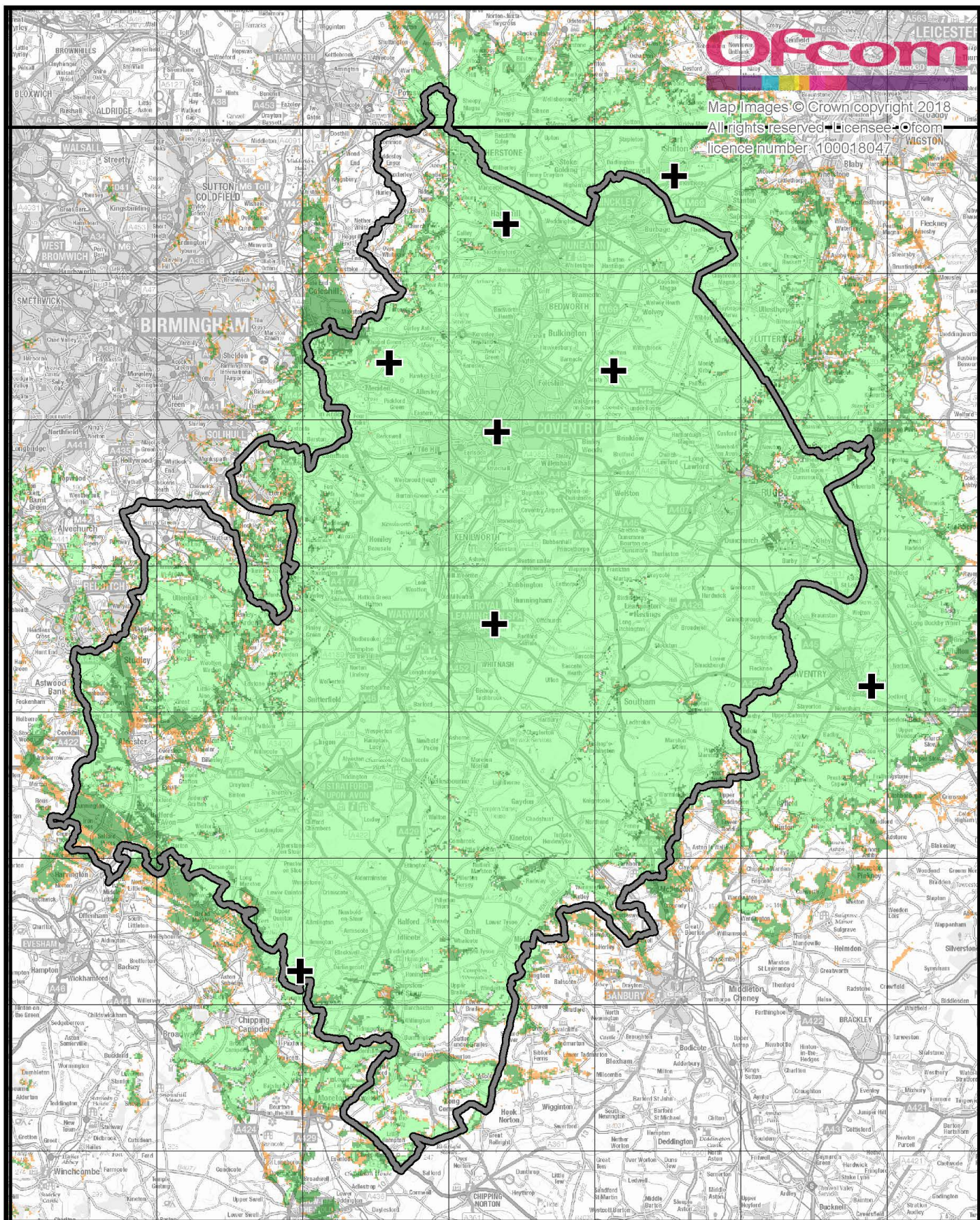
Coventry local DAB multiplex service (Now Digital). Indoor coverage, normal propagation conditions. July 2018.
