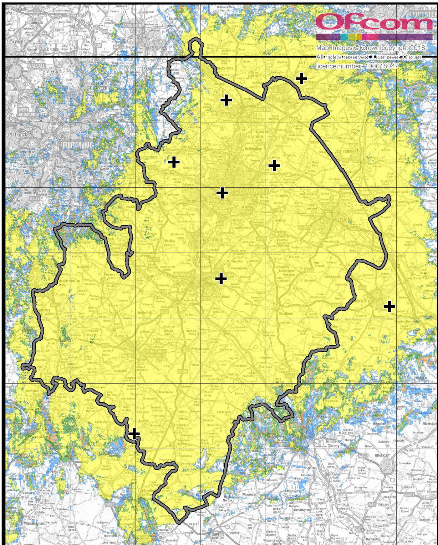
Coventry local DAB multiplex service (Now Digital). Mobile coverage, normal propagation conditions. July 2018.
