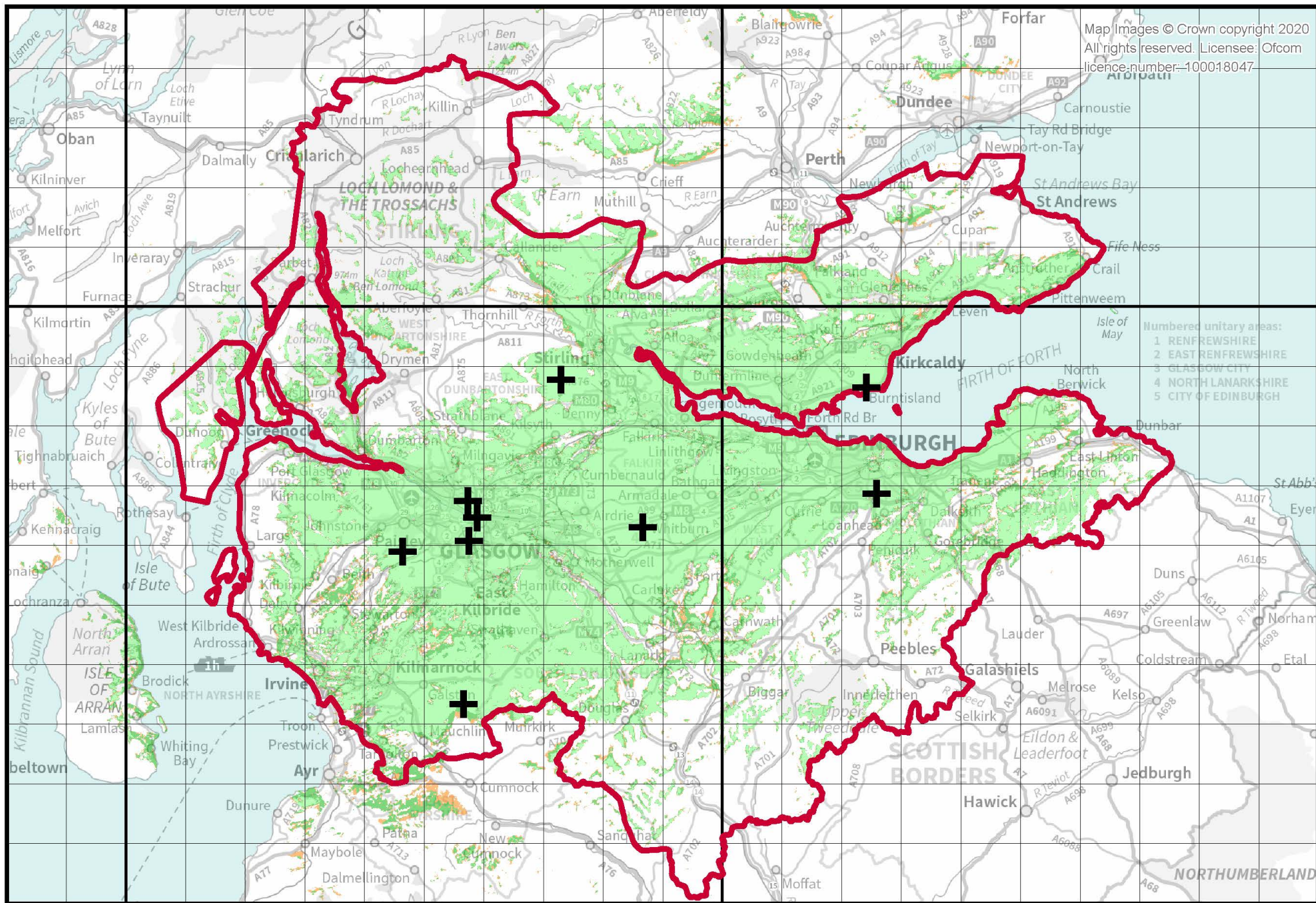
Central Scotland regional DAB multiplex service (Switch Digital) - Indoor coverage normal propagation conditions, January 2020
