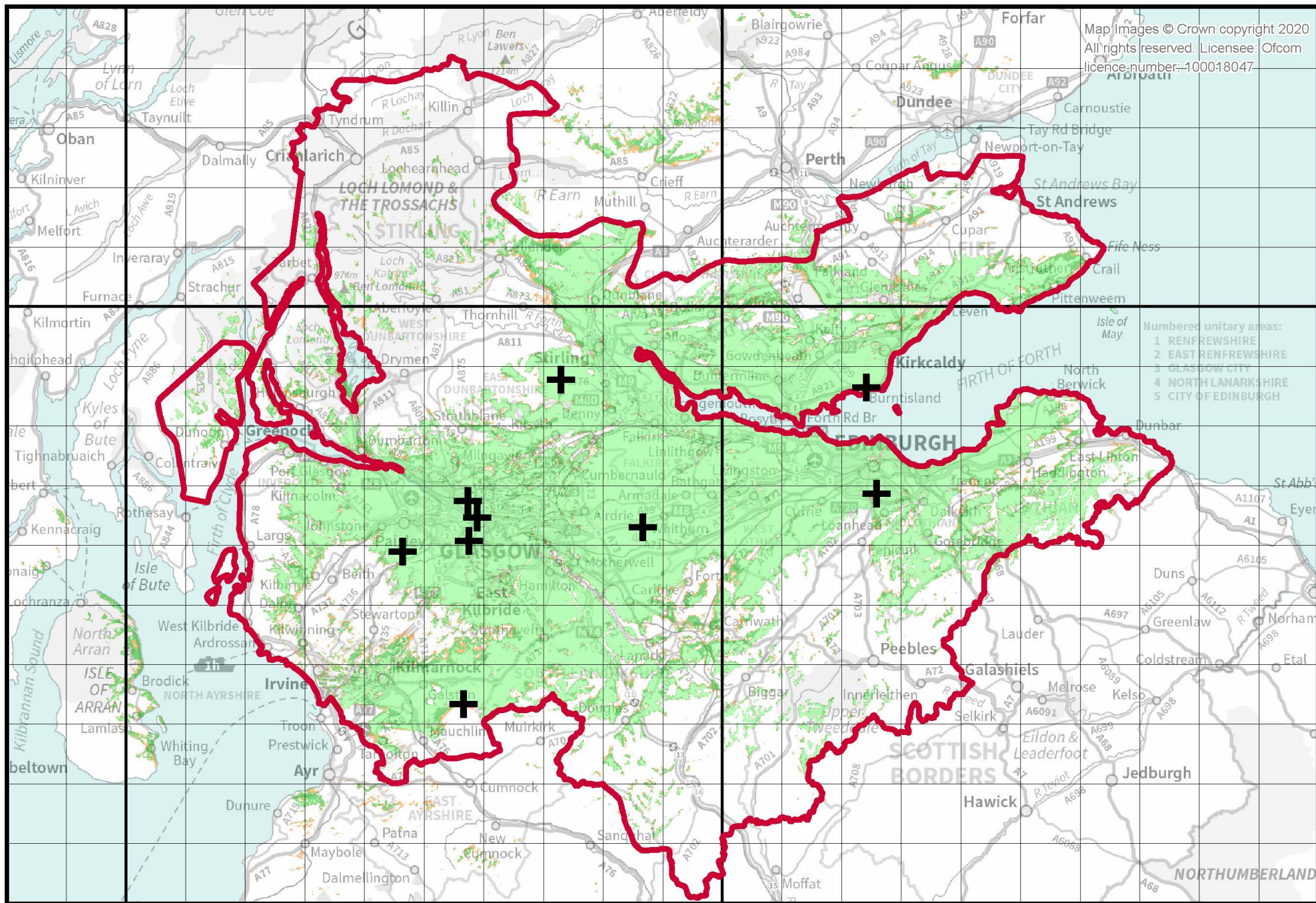
Central Scotland regional DAB multiplex service (Switch Digital) - Indoor coverage enhanced propagation conditions, January 2020
