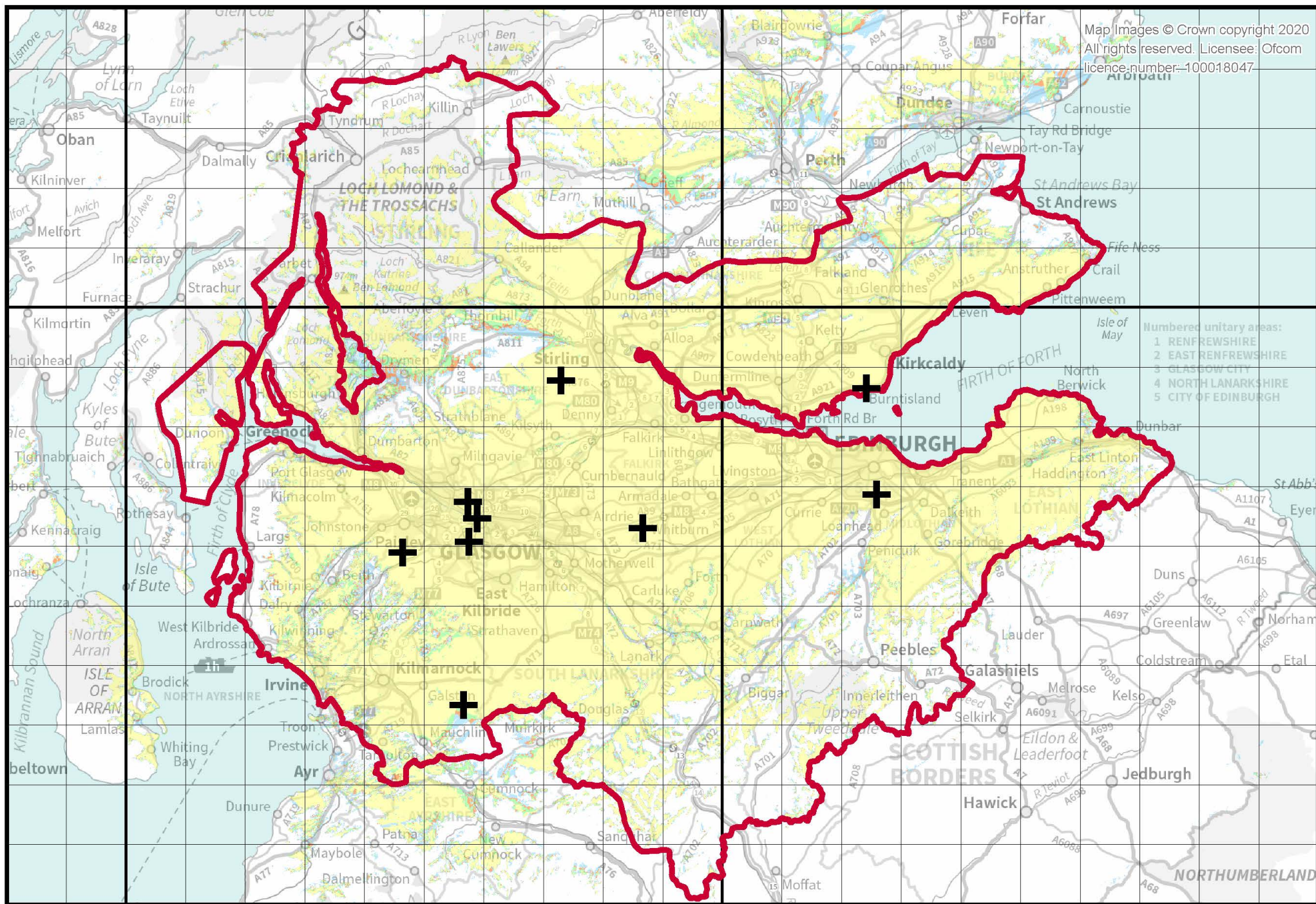
Central Scotland regional DAB multiplex service (Switch Digital) - Mobile coverage normal propagation conditions, January 2020
