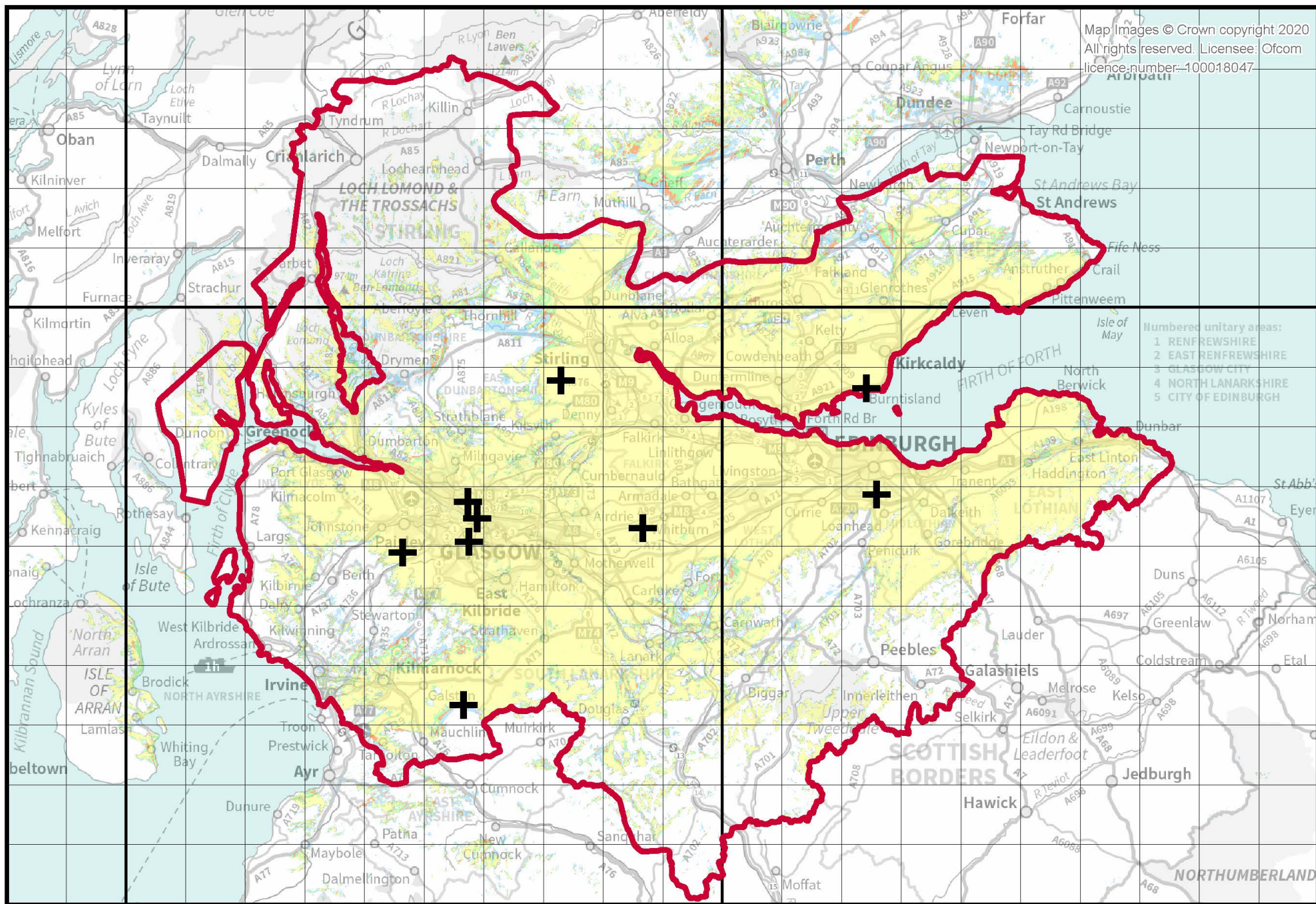
Central Scotland regional DAB multiplex service (Switch Digital) - Mobile coverage enhanced propagation conditions, January 2020
