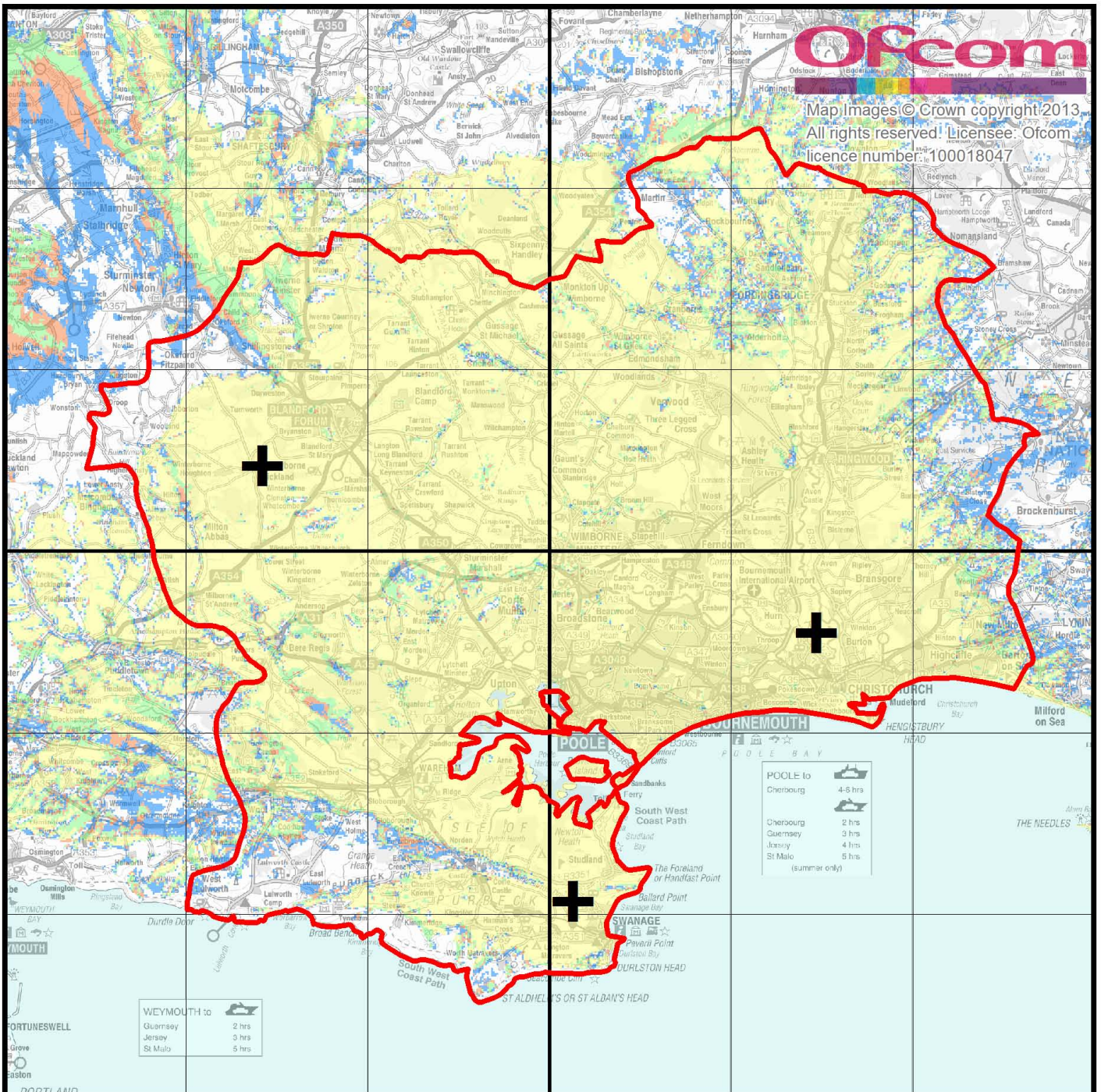
Bournemouth local DAB multiplex service (NOW Digital) mobile coverage normal propagation conditions, January 2013
