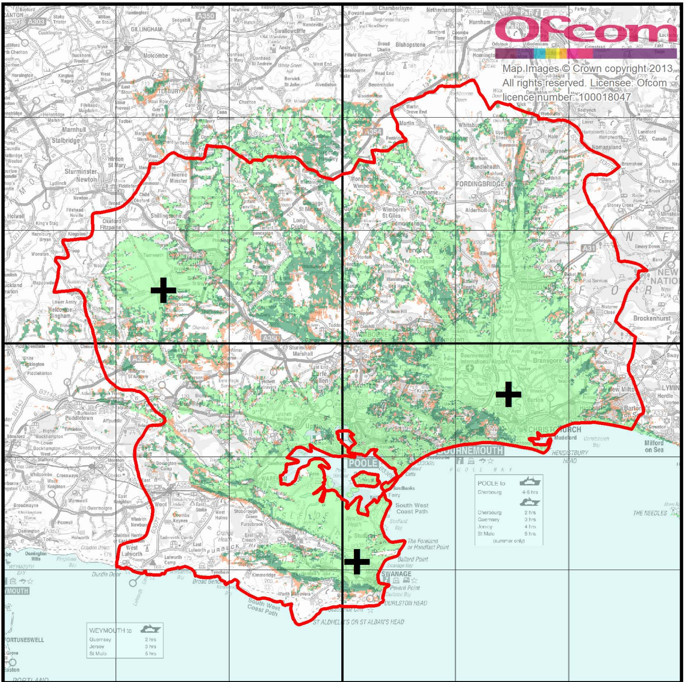
Bournemouth local DAB multiplex service (NOW Digital) indoor coverage enhanced propagation conditions, January 2013
