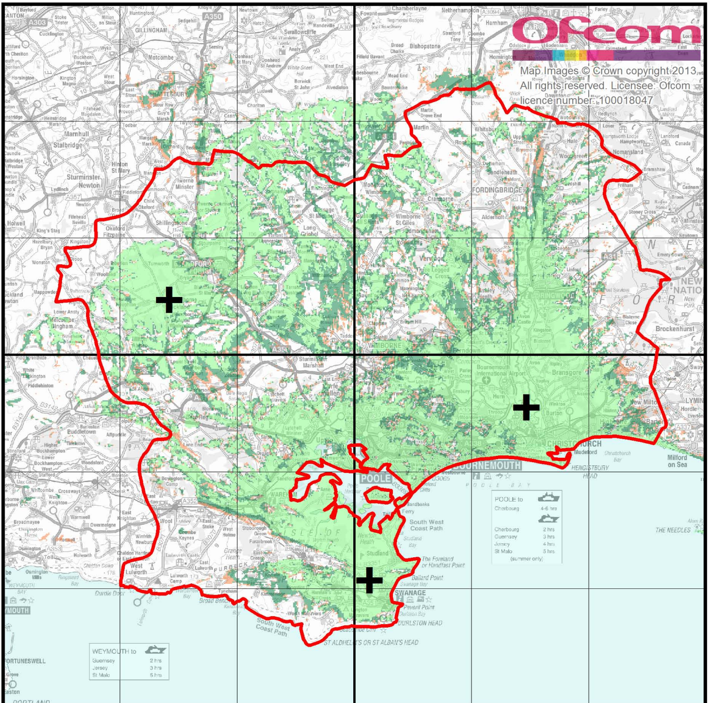
Bournemouth local DAB multiplex service (NOW Digital) indoor coverage normal propagation conditions, January 2013
