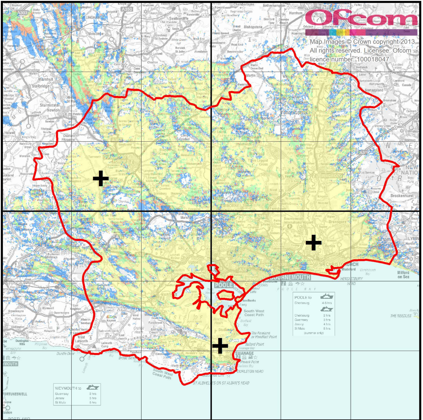
Bournemouth local DAB multiplex service (NOW Digital) mobile coverage enhanced propagation conditions, January 2013
