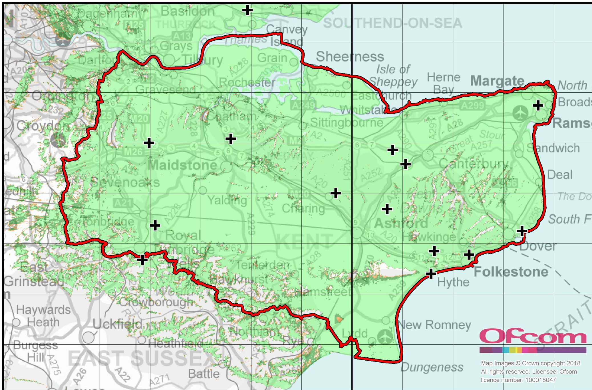
Kent local DAB multiplex service (NowDigital). Indoor coverage, normal propagation conditions. September 2018.
