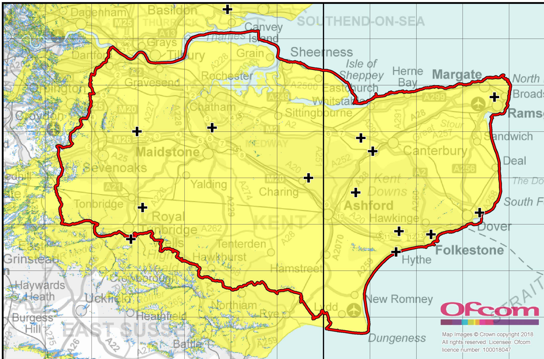
Kent local DAB multiplex service (NowDigital). Mobile coverage, normal propagation conditions. September 2018.
