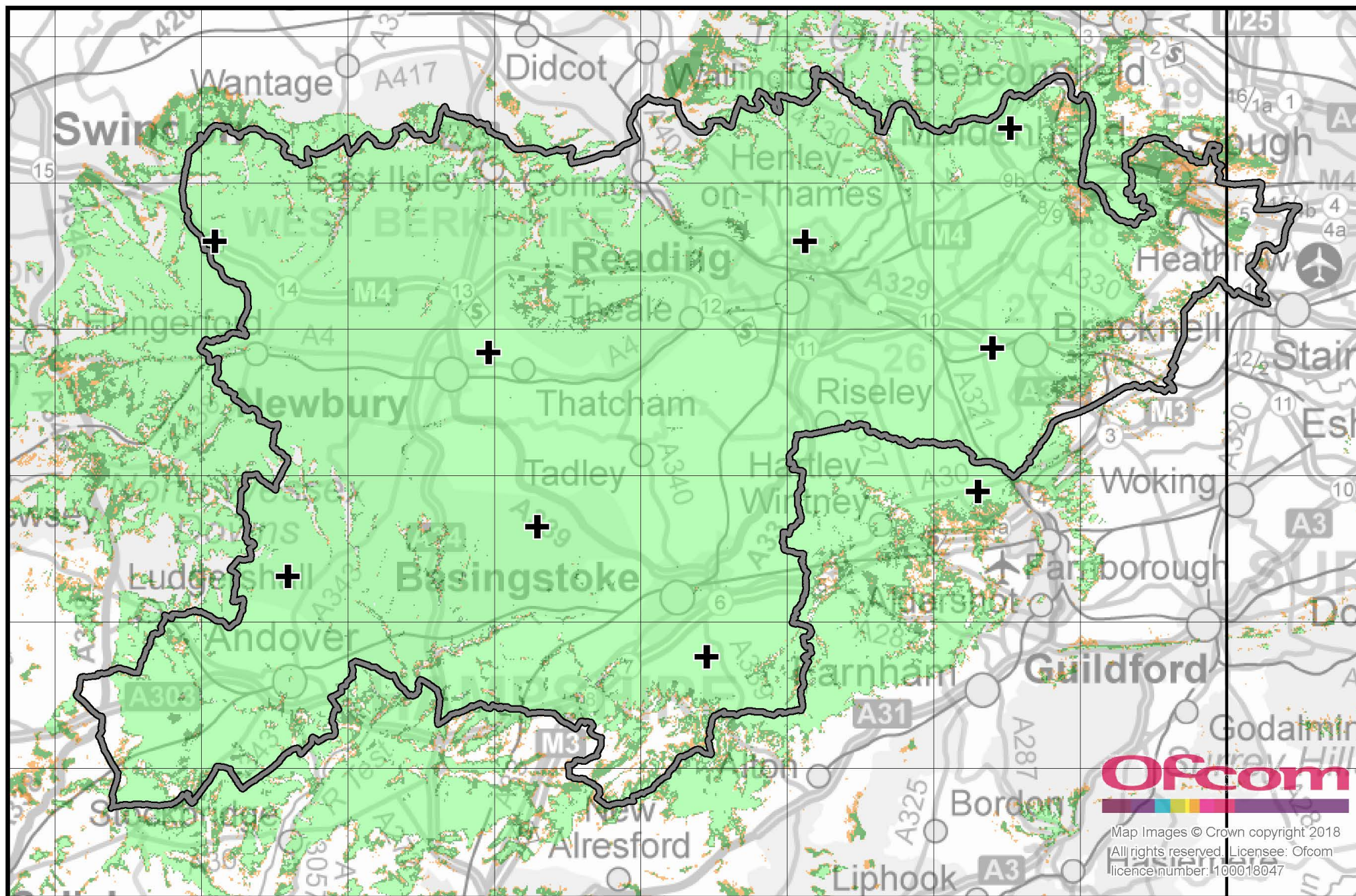
Berkshire & North Hampshire local DAB multiplex service (NowDigital). Indoor coverage, normal propagation conditions. July 2018.
