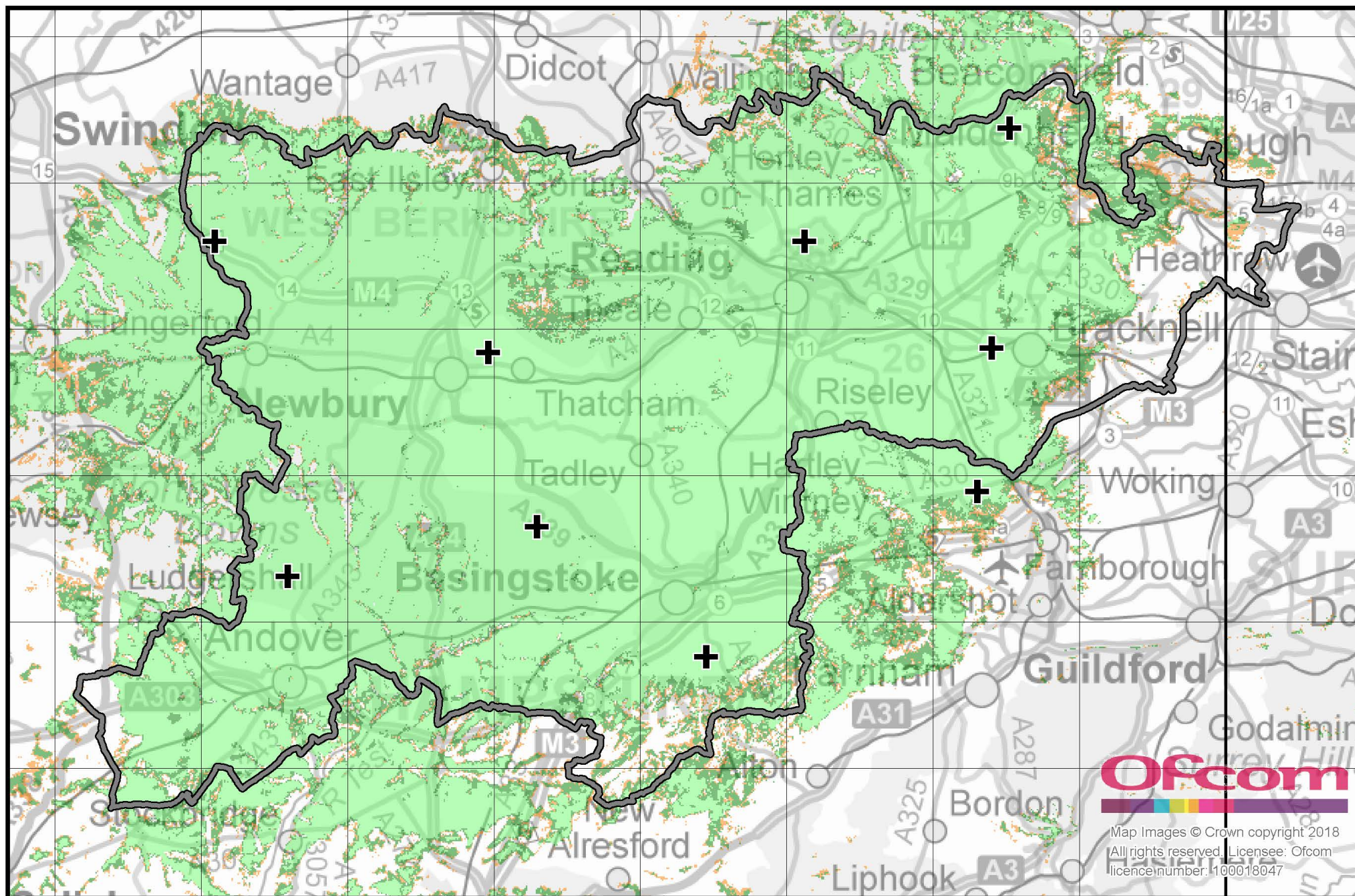
Berkshire & North Hampshire local DAB multiplex service (NowDigital). Indoor coverage, enhanced propagation conditions. July 2018.
