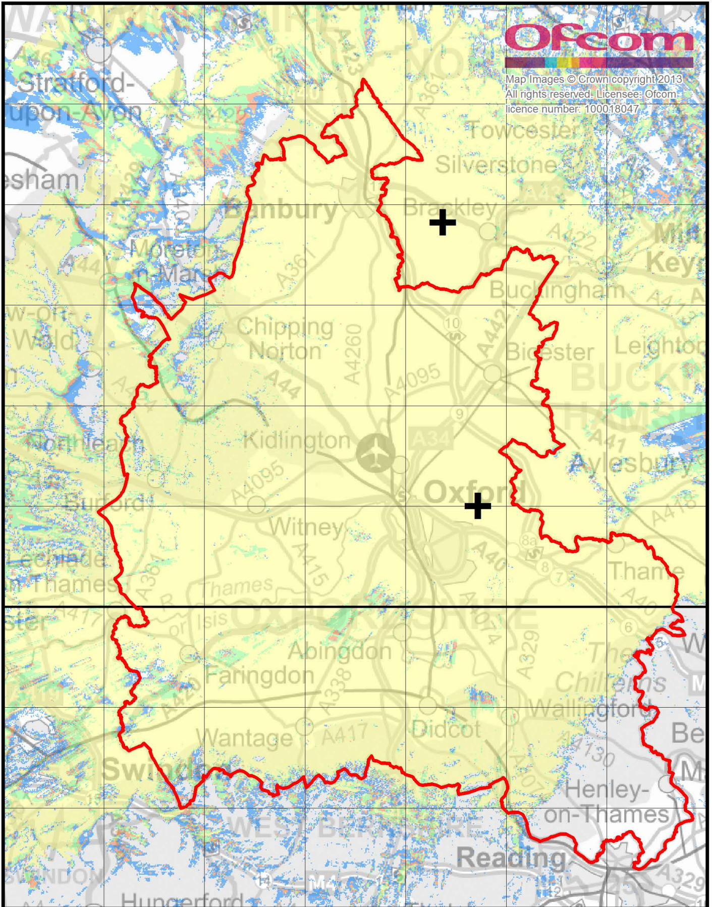
Oxfordshire local DAB multiplex service (NOW Digital) mobile coverage normal propagation conditions, January 2013
