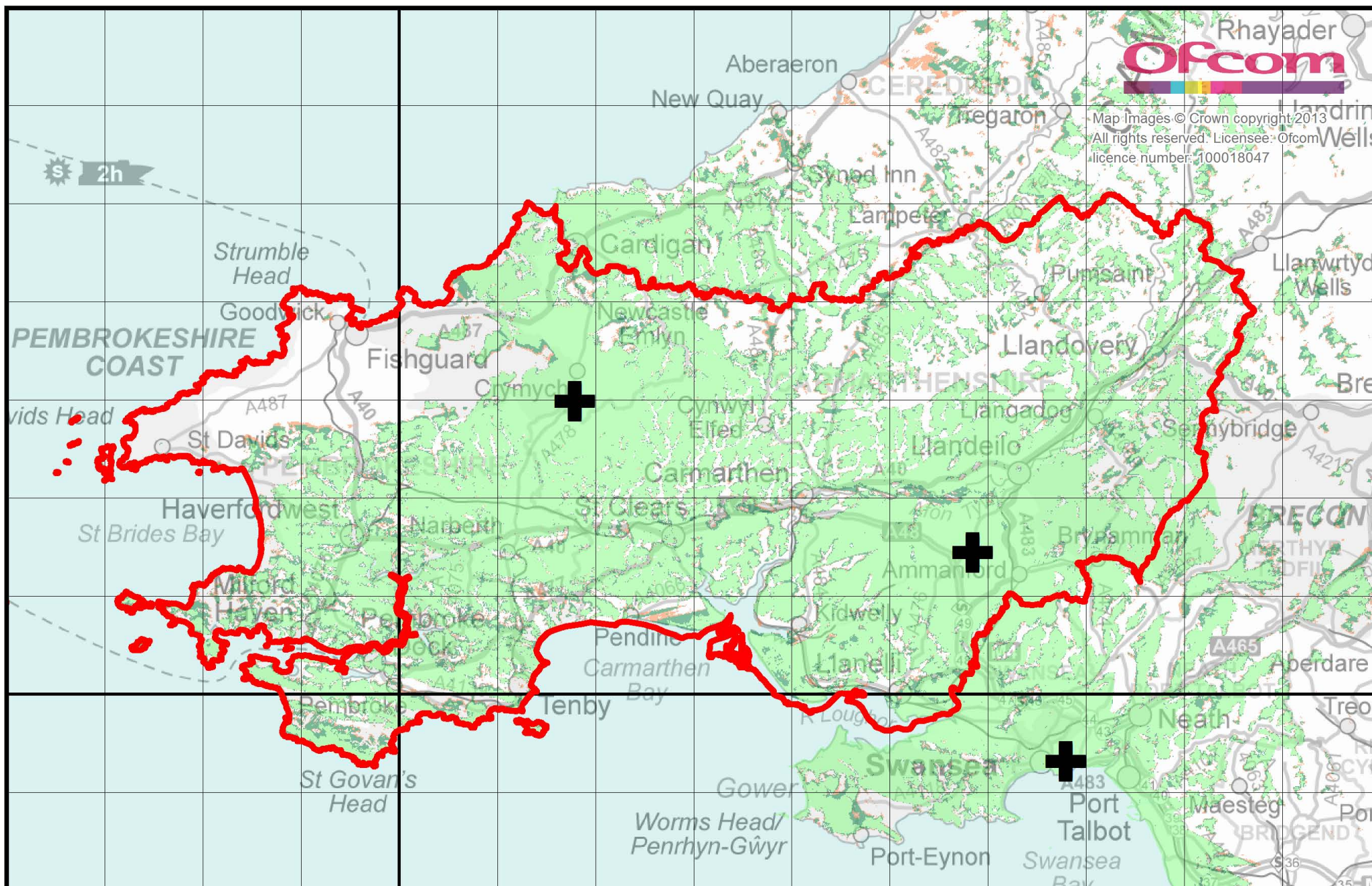
Mid and West Wales local DAB multiplex service (MuxCo) indoor coverage normal propagation conditions, September 2013
