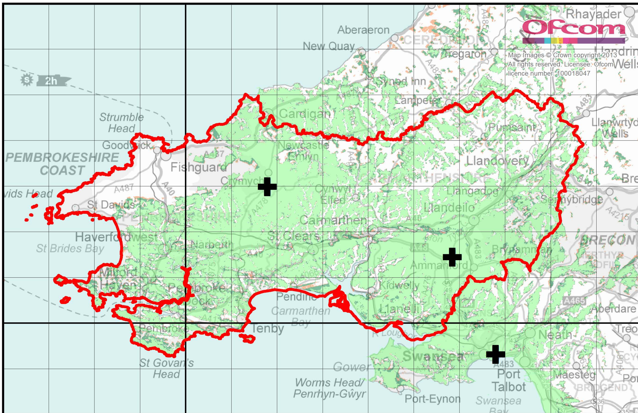
Mid and West Wales local DAB multiplex service (MuxCo) indoor coverage enhanced propagation conditions, September 2013
