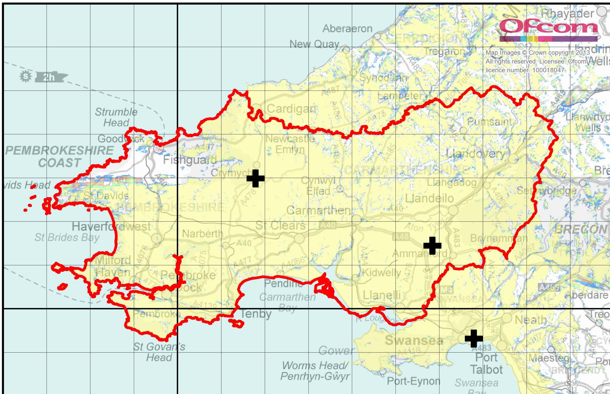
Mid and West Wales local DAB multiplex service (MuxCo) mobile coverage enhanced propagation conditions, September 2013
